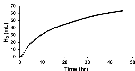
Figure 4. \text{H}_2 production profile using [(\text{Ph}_2\text{phen})_2\text{Ru}(\text{dpp})]_2\text{RhBr}_2^{5+} (120 \mu\text{M} ) in \text{DMF} photolyzed at 460 nm in the presence of \text{H}_2\text{O} (0.62 M) and the electron donor DMA (3.1 M).
